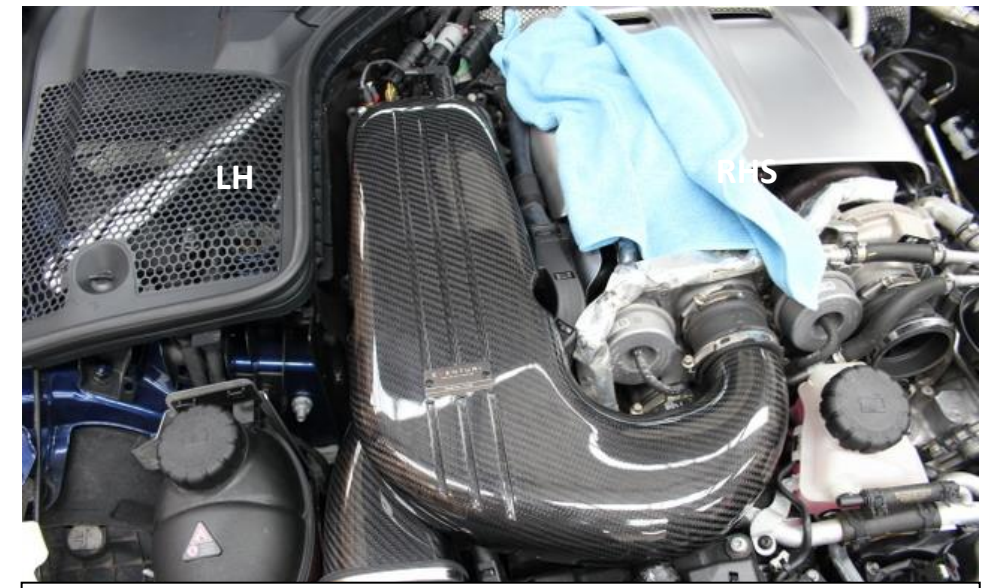
24. Carefully rotate the lid downwards onto the airbox base. The rubber mount under the lid should go onto the mounting position.
