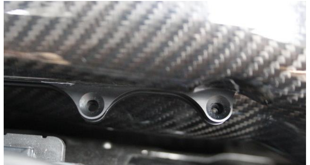
26. The flanges should line so that the holes are all in line.
