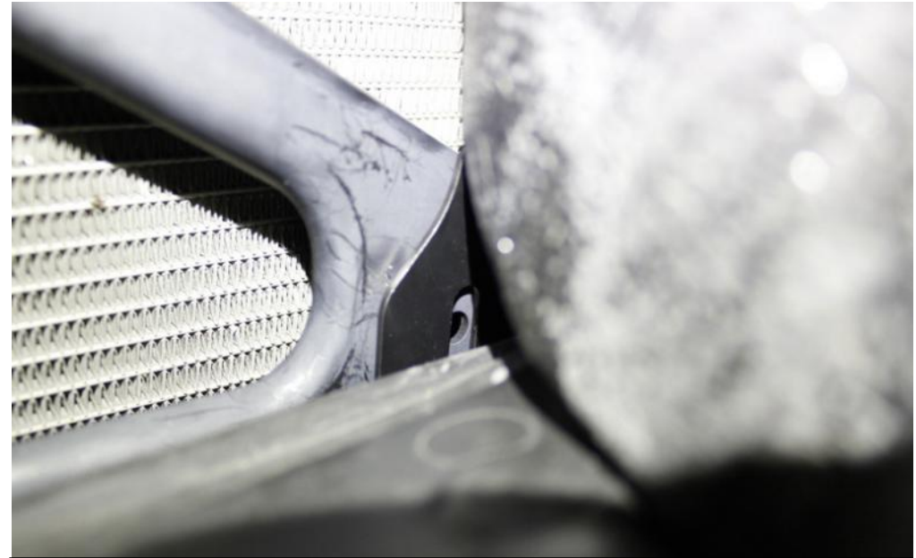
61. As previously, align the bracket with the hole on the strut brace and secure with the push rivet.
