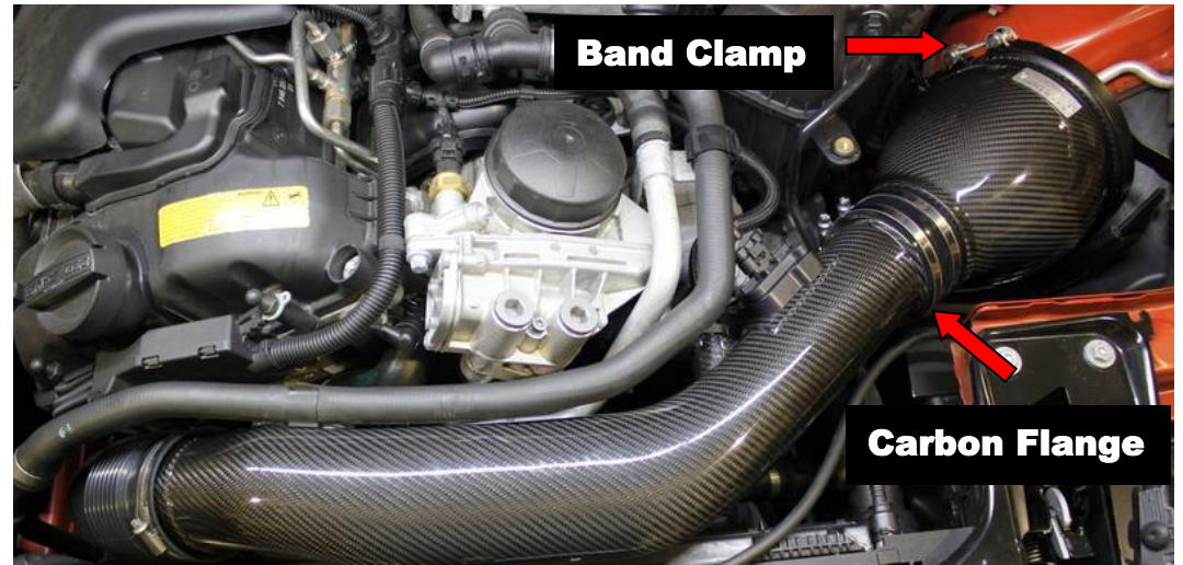
46. Once positioned correctly, tighten the hose clamps on both sides of the carbon tube. Ensure there is no gap between the flange on the carbon and the silicon as shown. Tighten the Band Clamp holding the filter and housing together. Reinstall strut brace with all 13mm bolts and the 10mm bolt.
