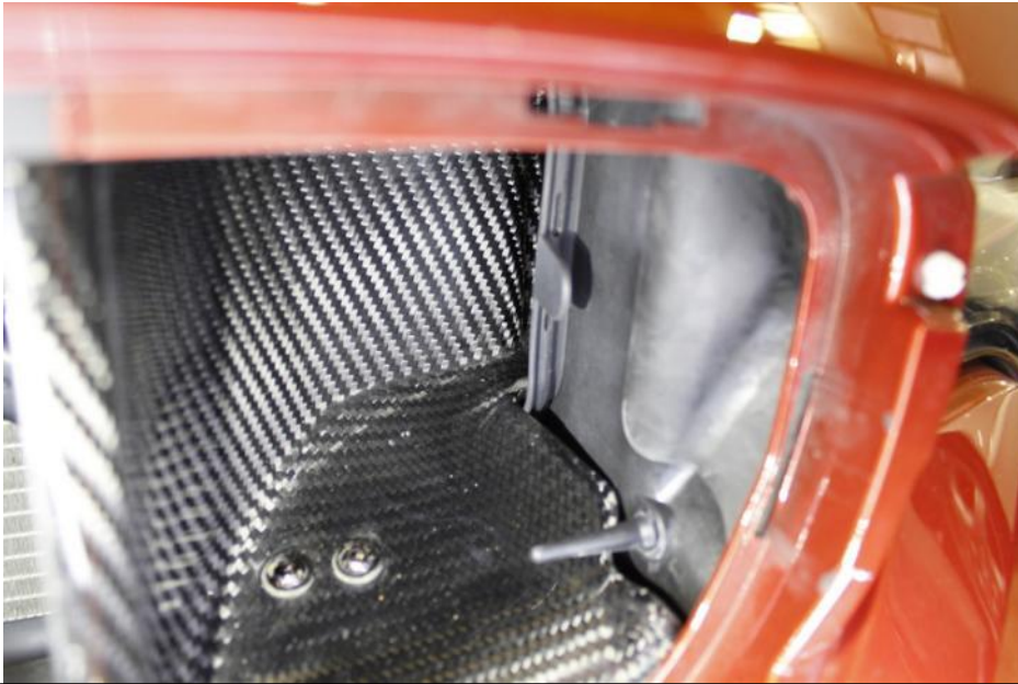
60. The back of the scoop should be positioned as shown inside the stock opening.
