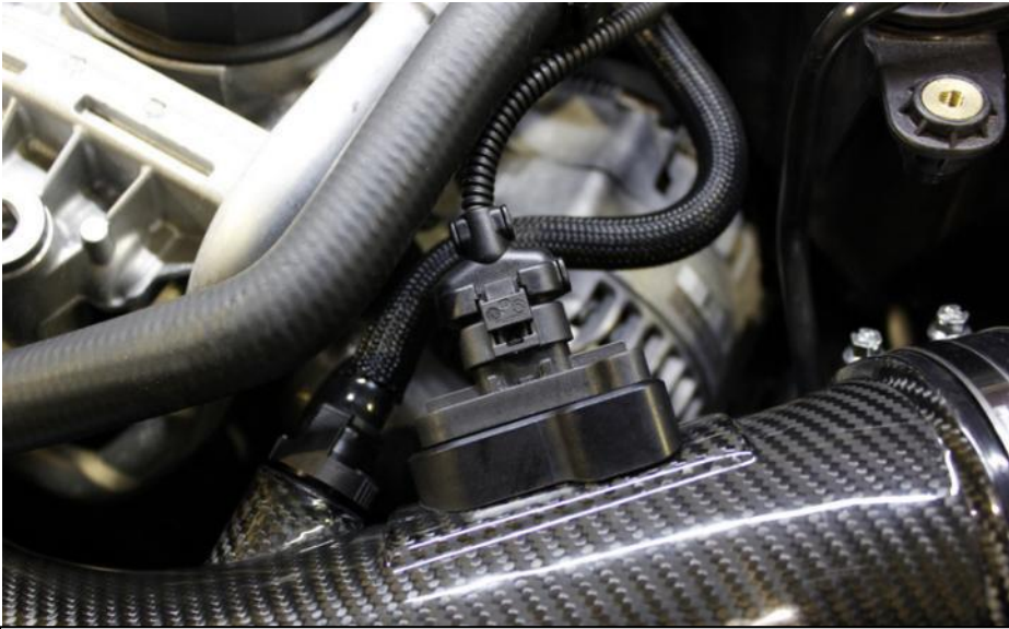
43. Insert breather tube into place – it should click into place. Reconnect MAF sensor plug ensuring it has engaged fully.
