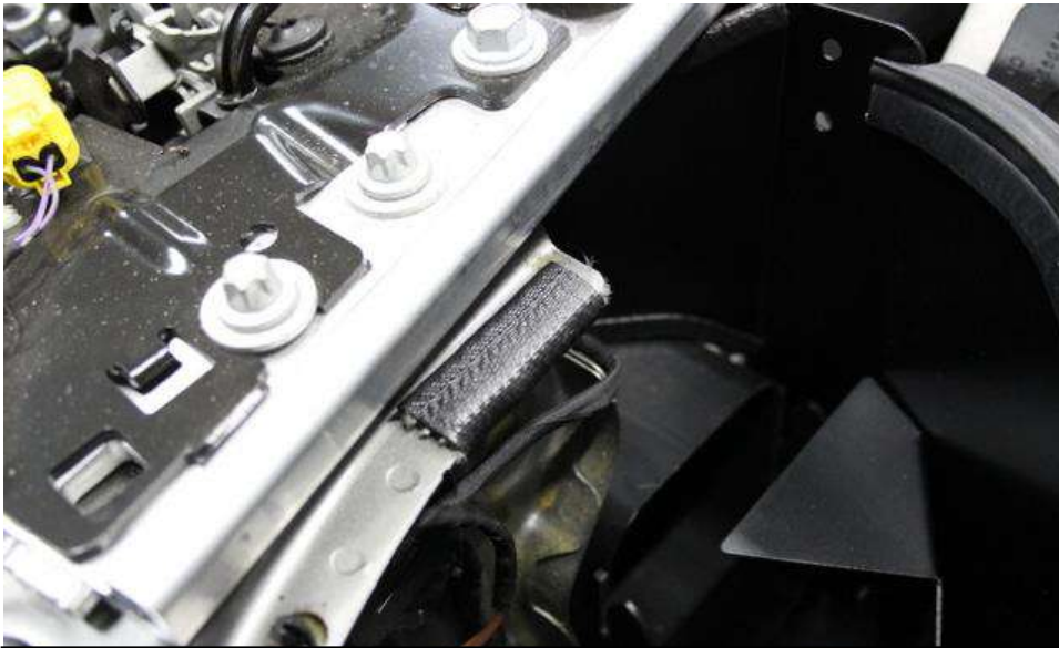
33. Close-up view of the edging installed in the right side. Now install the RHS housing in the same way as the LHS housing.
