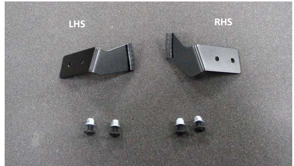
34. With both housings installed – we will now secure the shields. Take the supplied brackets and M5 screws with lock nuts. Identify the LHS and RHS.
