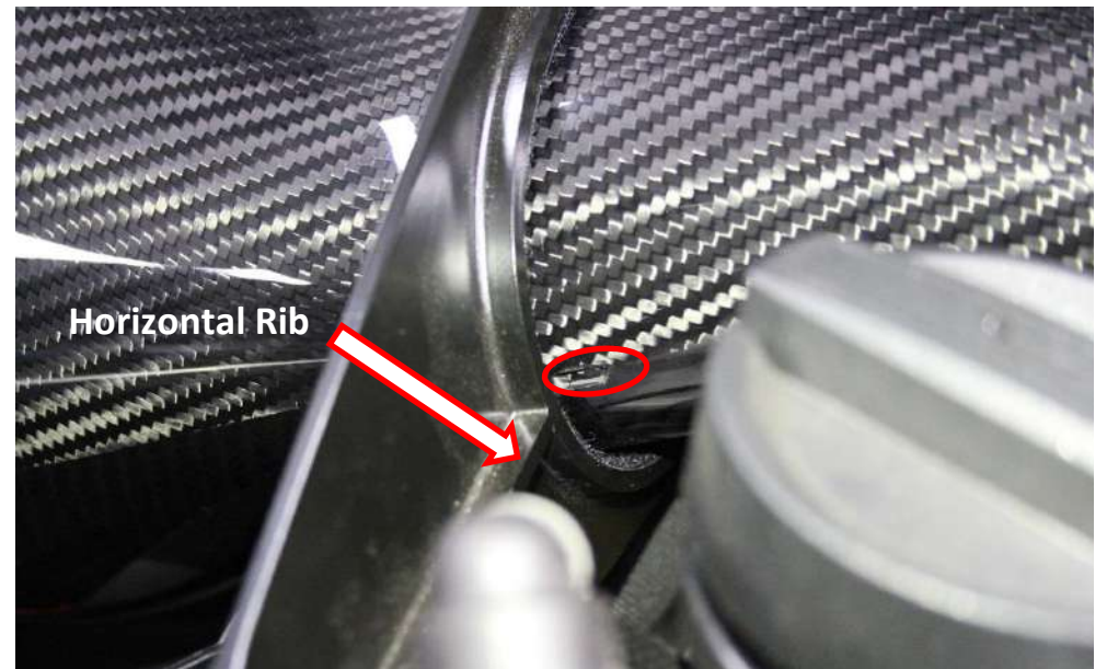
28. Rotate the housing so that the notch in the carbon circled red lines up with the horizontal rib on the strut brace as shown.
