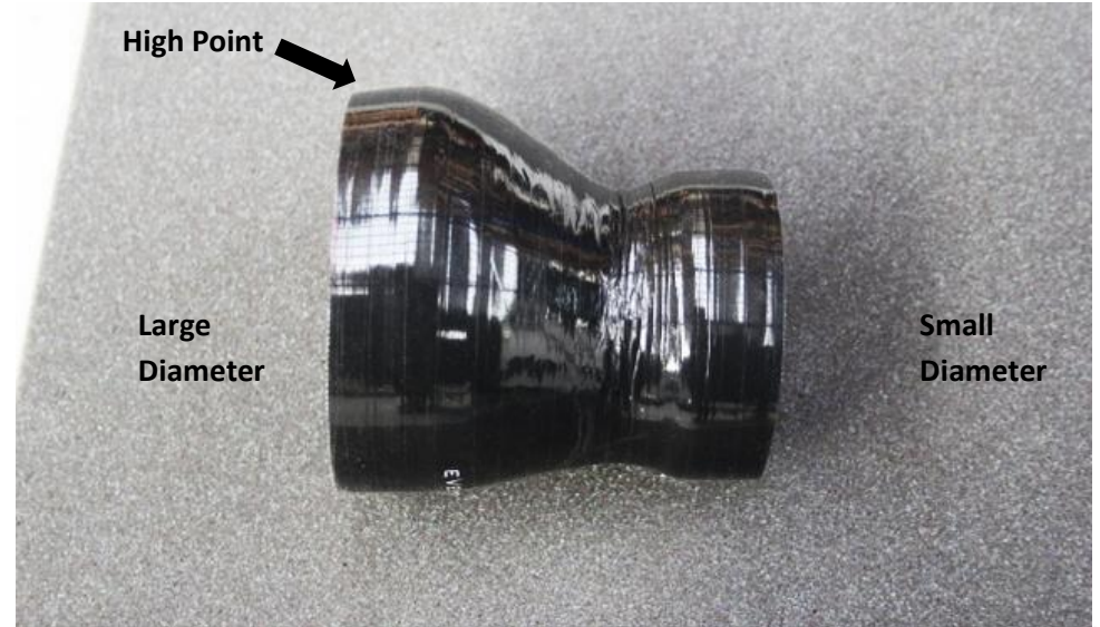
21. Take the silicon reducer – notice the large diameter side is offset from the small diameter – it is not symmetrical. Rotate the hose until the highest point of the large diameter side is at the top as shown.
