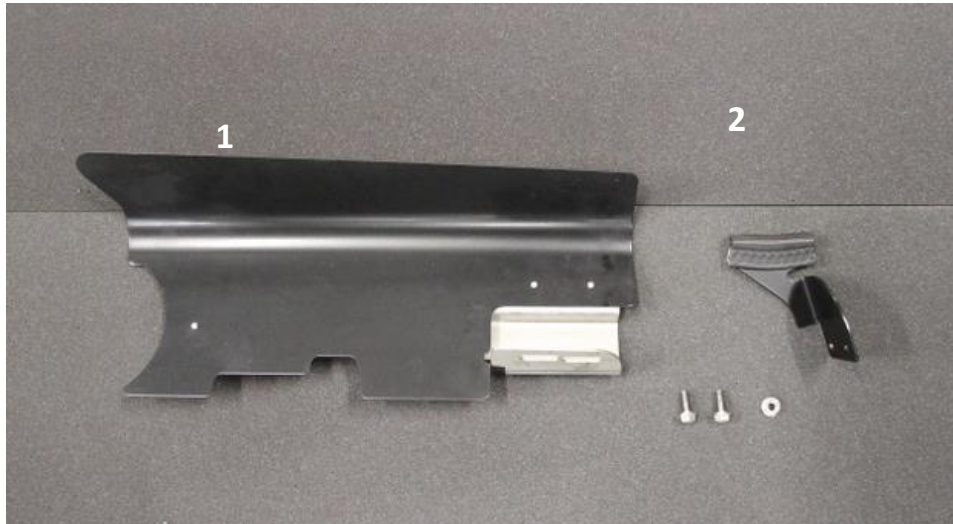
16. Take the heat shield, tube bracket with rubber edge and the 2 supplied M6 Screws with 1 M6 Non Locking Nut.
