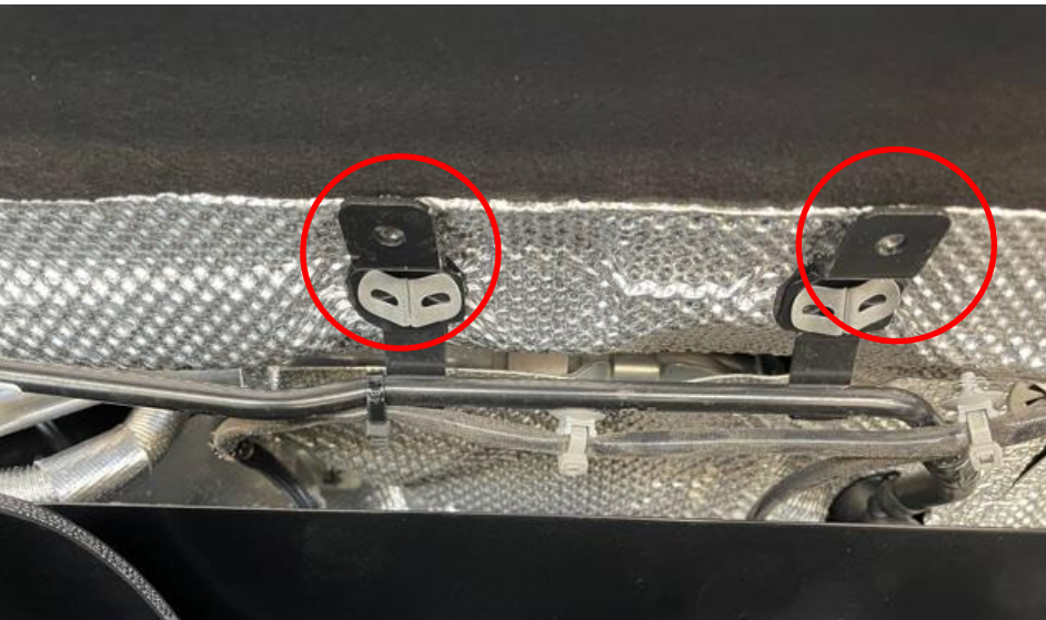
14. Unclip the grey wire harness clips from the metal brackets and tie the harness to the tube underneath.
