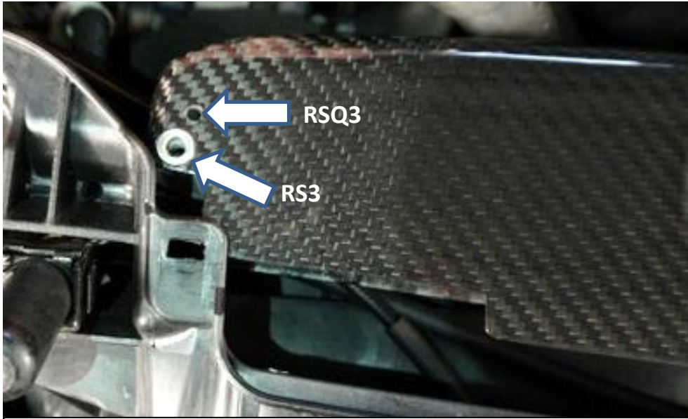
40. Before securing identify the correct holes to use on the duct. The hole with the insert is for the RS3 – the plain smaller hole above it is only for the RSQ3.
