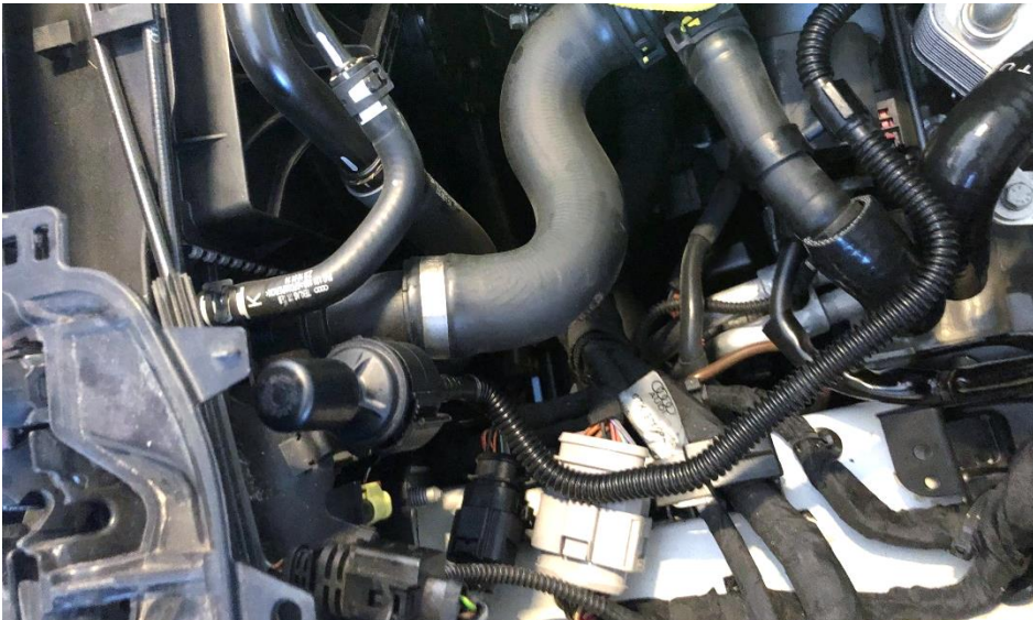
20. Route the Oil breather pot to the panel behind the headlamp – make sure the oil line is routed as shown
