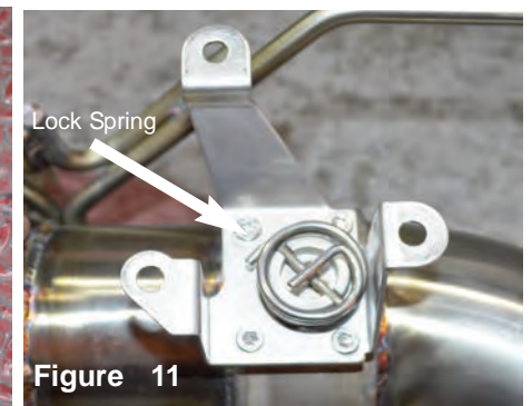
Figure 11 Now install the provided Lock spring and position to the new motor housing like above image.
