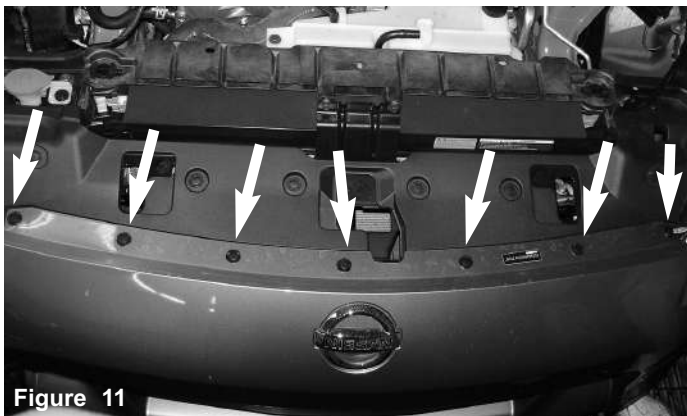
Figure 11 The 7 plastic tabs to be removed from the upper bumper lip.
