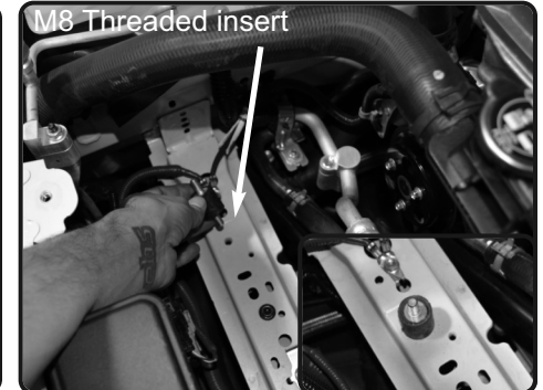
7. Install the M8 vibramount to the threaded insert on frame. Secure and tighten.
