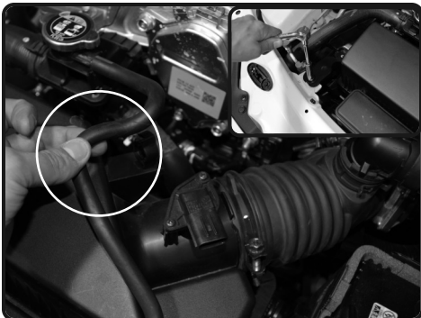
4. With 10mm socket and extension and ratchet, loosen the screw holding in the airbox on radiator support and clamp on throttle body. Pull back the coolant line from air box. Save screw for later install.
