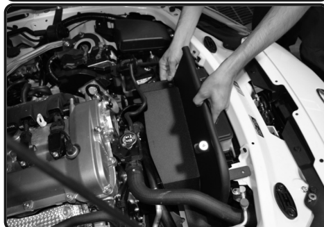
9. Install the heatshield into the vehicle. Position the grommet on heatshield to original air box fitting.
