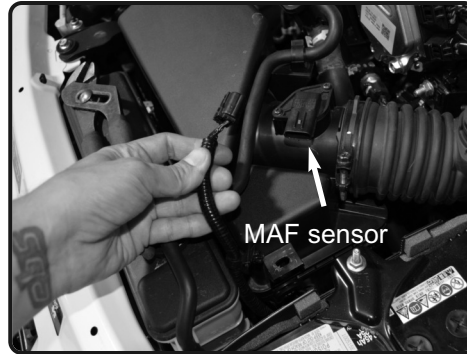
2. Disconnect the MAF sensor harness.
