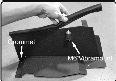
8. Install the Rubber trim to the top of heatshield. Install the M6 vibramount to the tab with threaded insert and secure. Install grommet to hole on heat shield.
