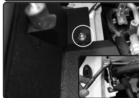
10. Secure the hole on heatshield to the M8 vibramount using provided M8 nut and washer. Secure the bracket using original screw from airbox and tighten.
