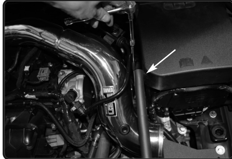
22. Secure the stand off stud using provided M6 nut and fender washer. Secure and tighten using 10mm socket and ratchet.
